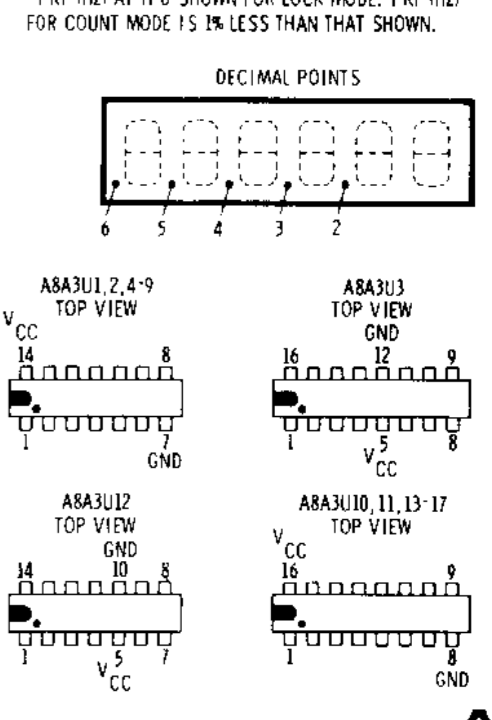
Figure 8-64. Counter Time Base Schematic Diagram
