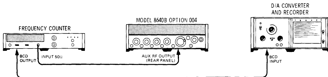
Figure 4-1. Frequency Stability us Time and Restabilization Time Test Setup
