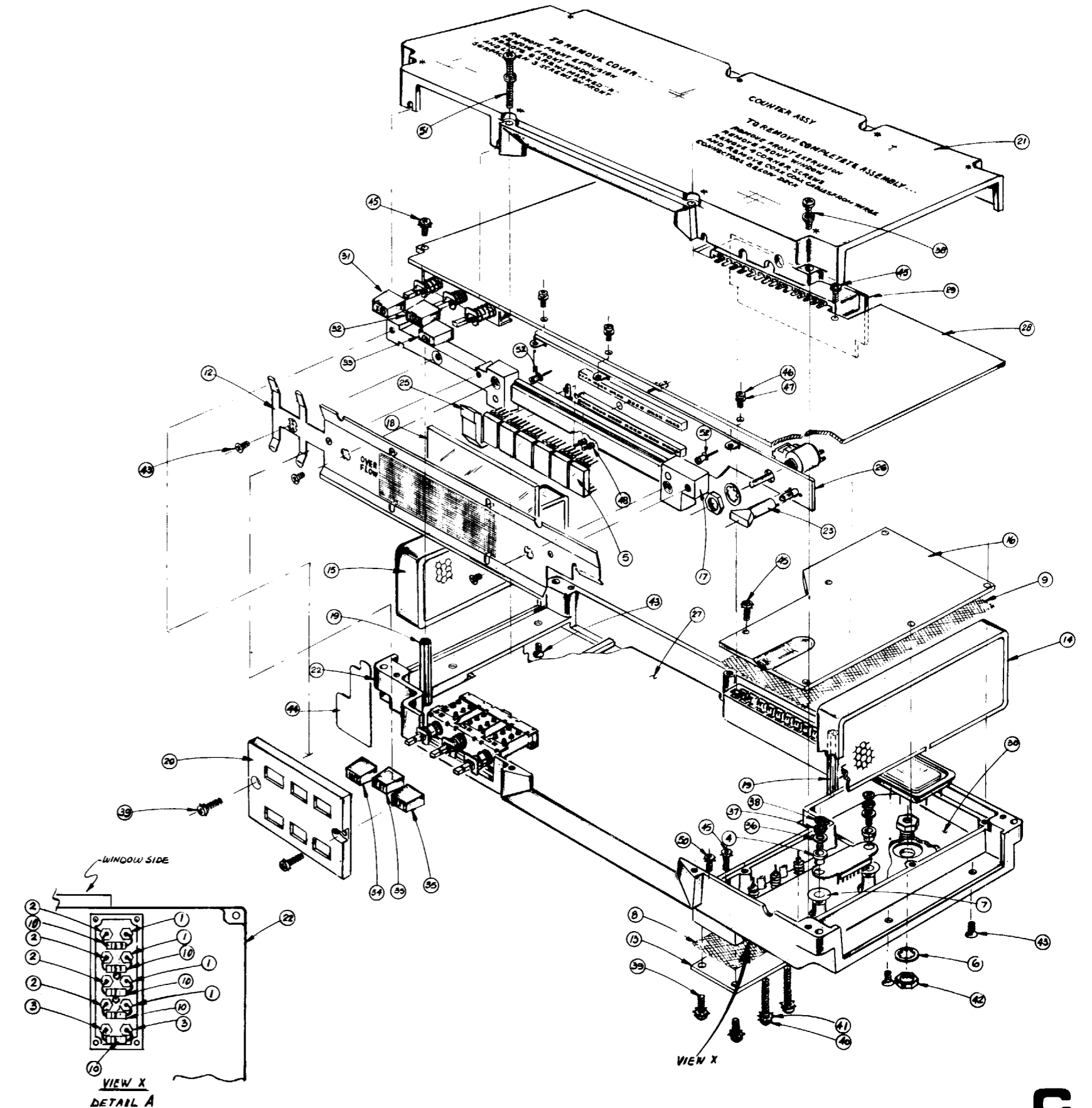
Figure 8-85. A8 Counter/Lock Assembly Illustrated Parts Breakdown
