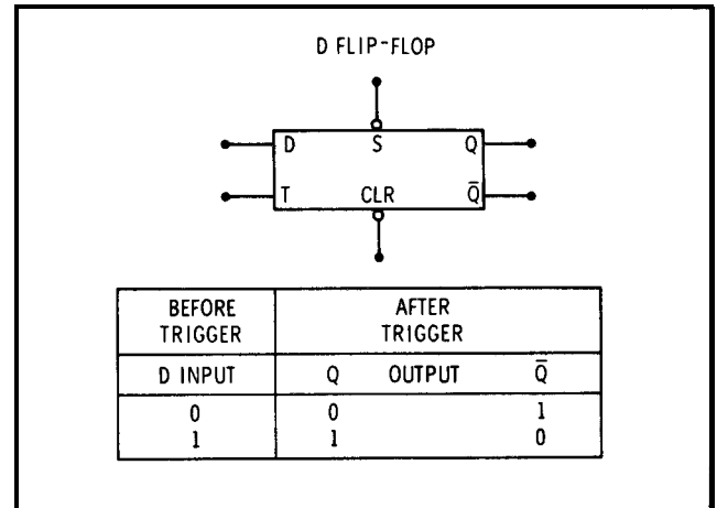
Figure 8-6. D Flip-Flop
