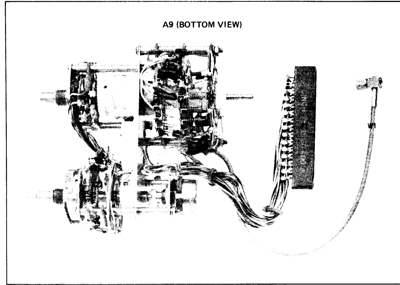
Figure 8-31. P/O A9 Peak Deviation and Range Switch Assembly Component Locations (2 of 2)
