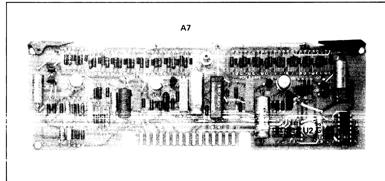
Figure 8-32. P/O A7 FM Shaping Assembly Component Locations
