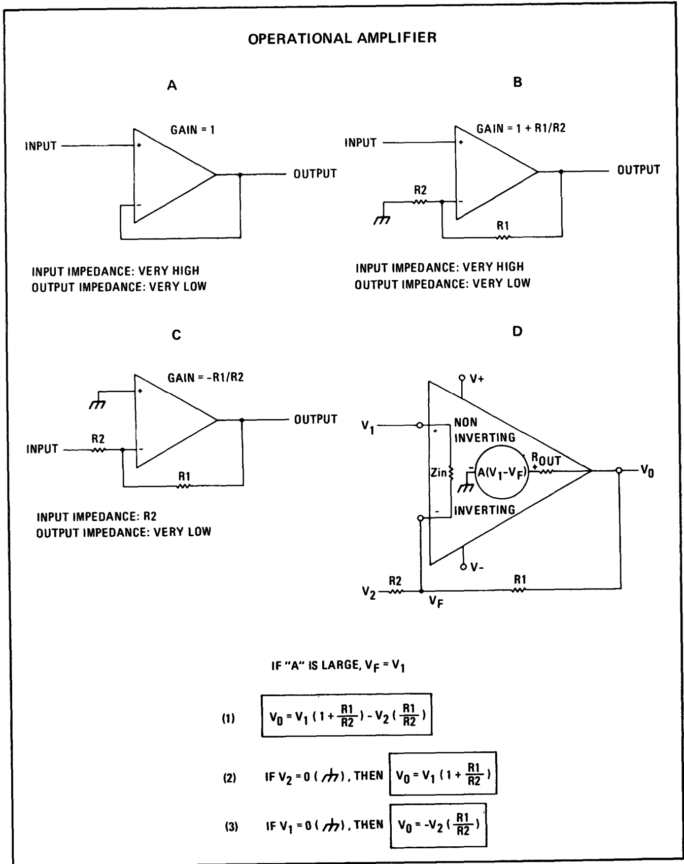
Figure 8-15. Operational Amplifier
