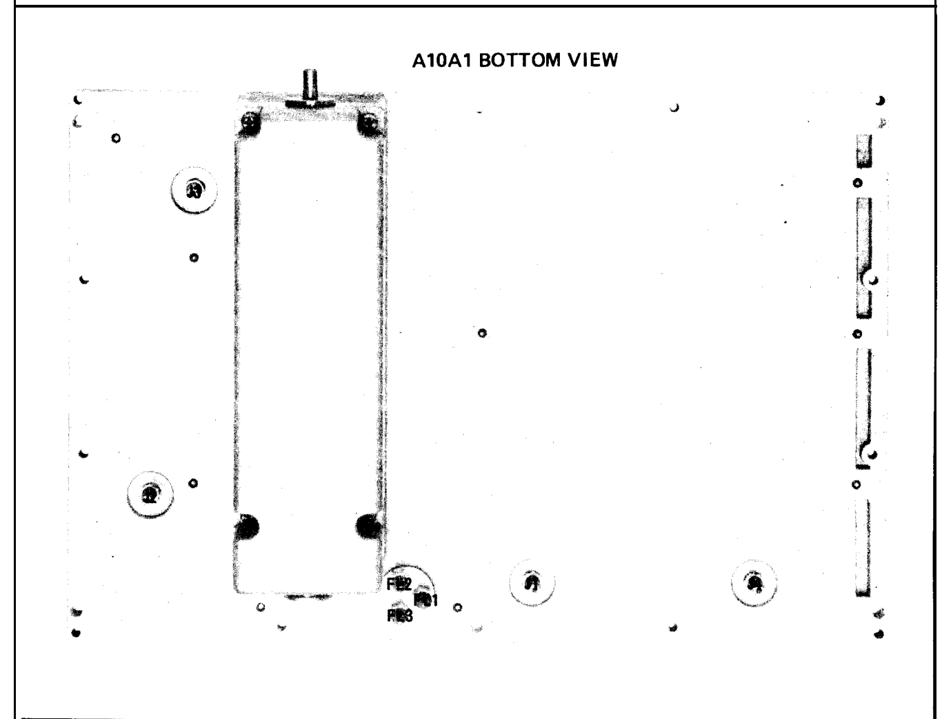
Figure 8-39. A10A1 RF Filter Assembly Component Locations (1 of 2)
