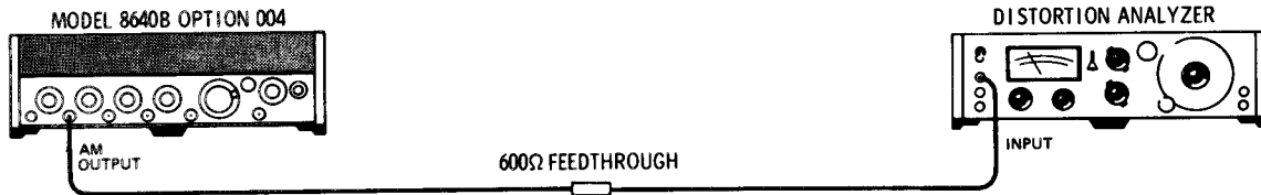
Figure 4-17. Internal Modulation Oscillator Distortion Test Setup
