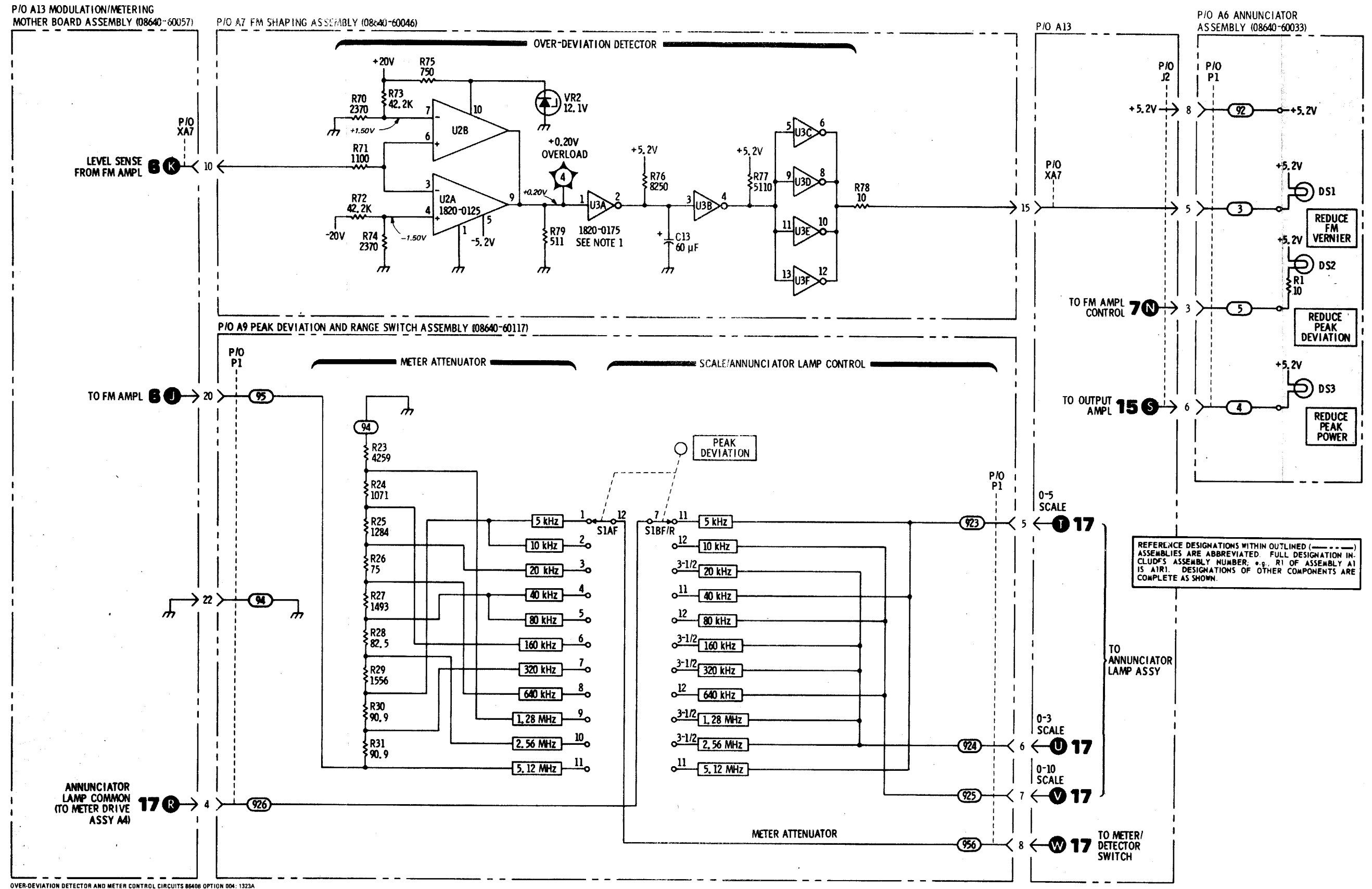
Figure 8-33. Over-Deviation Detector and Meter Control Circuits Schematic Diagram
