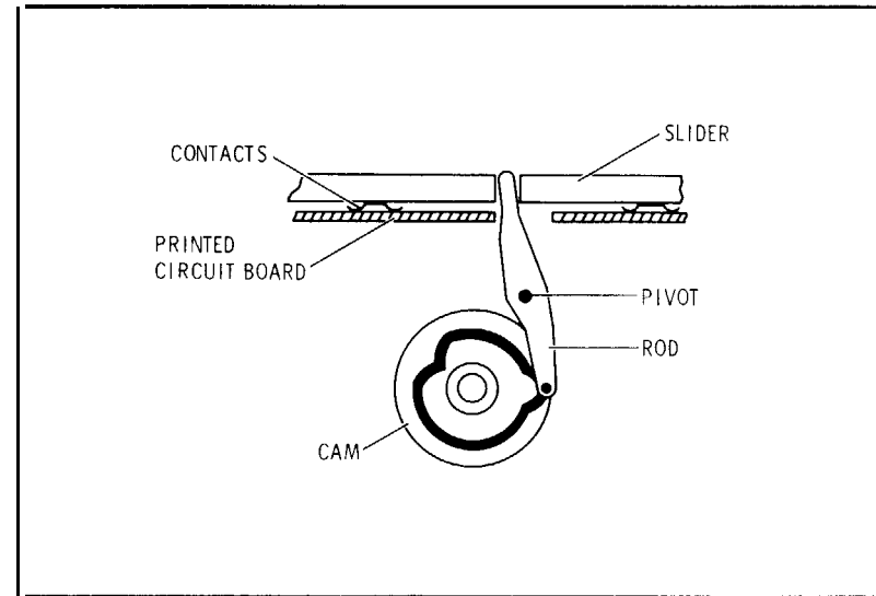
Figure 8-38. Action of RANGE Switch
