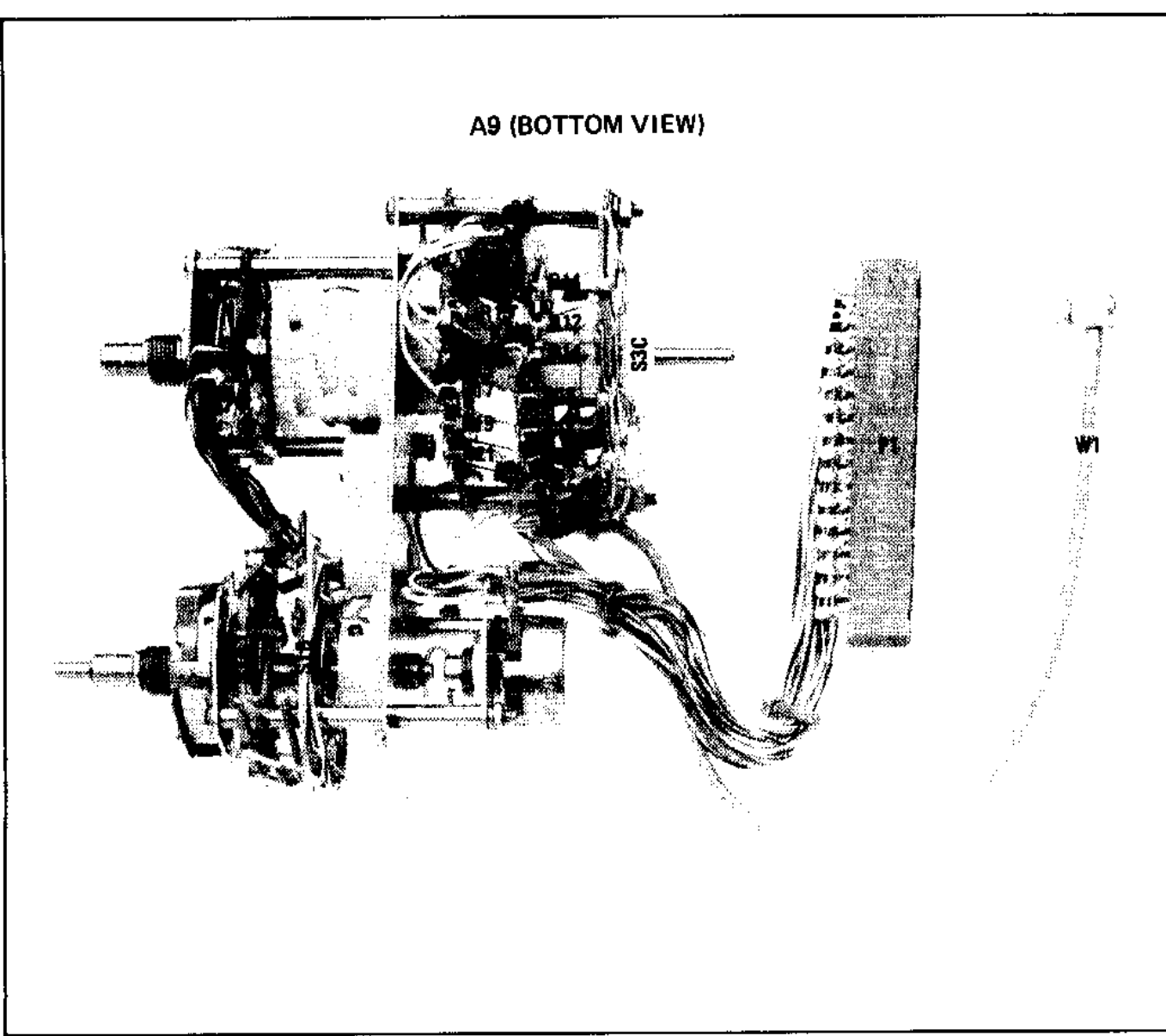
Figure 8-25. P/O A9 Peak Deviation and Range Switch Assembly Component Locations (2 of 2)
