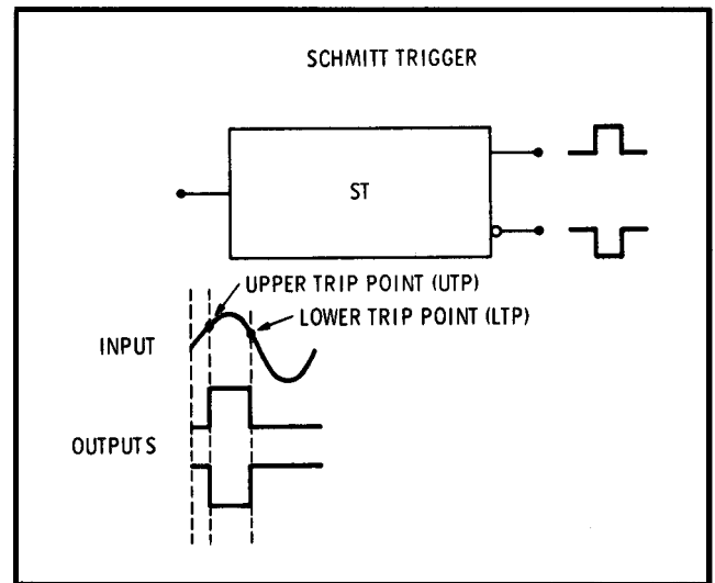
Figure 8-7. Schmitt Trigger
