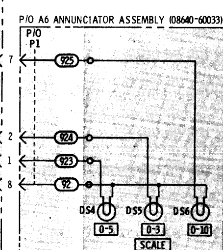
Figure 8-59. Meter Circuits Schematic Diagram
