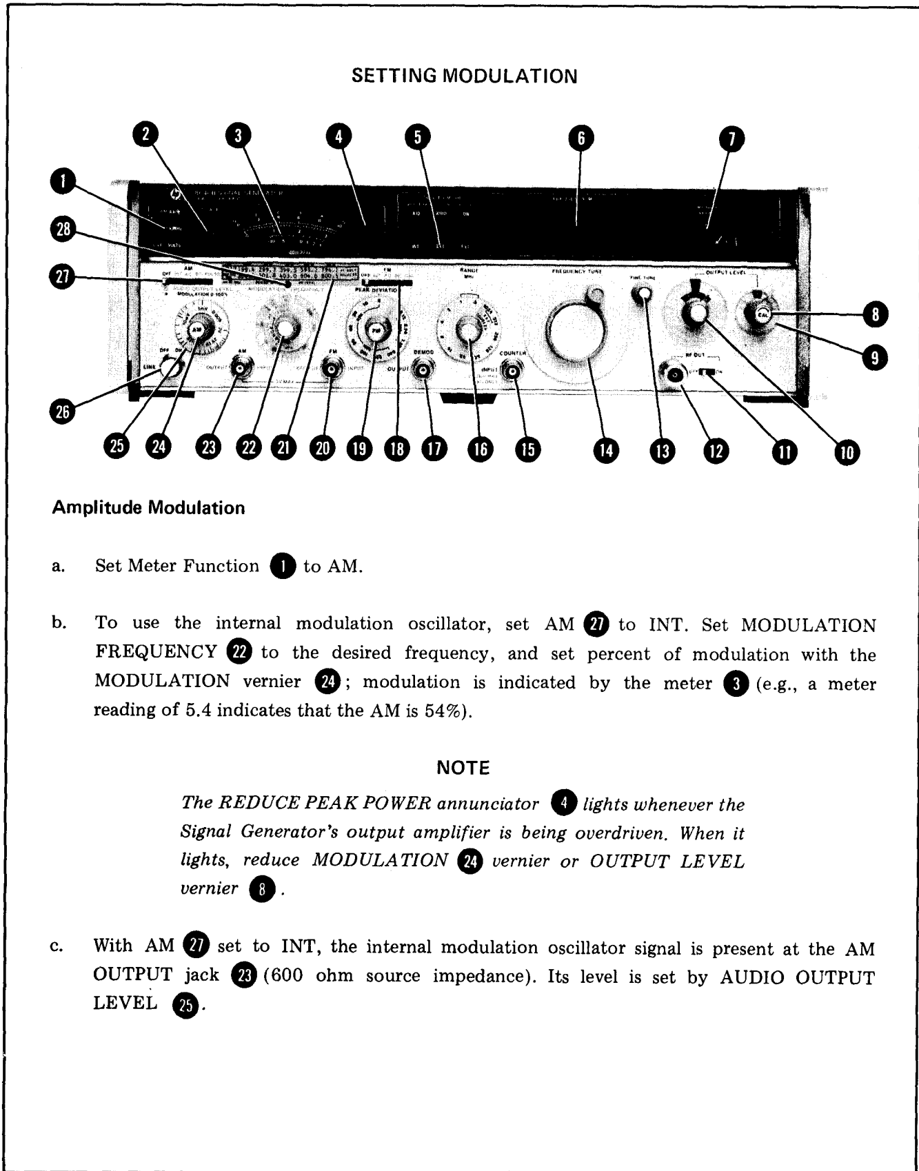
Figure 3-7. Setting the Modulation Controls (1 of 5)
