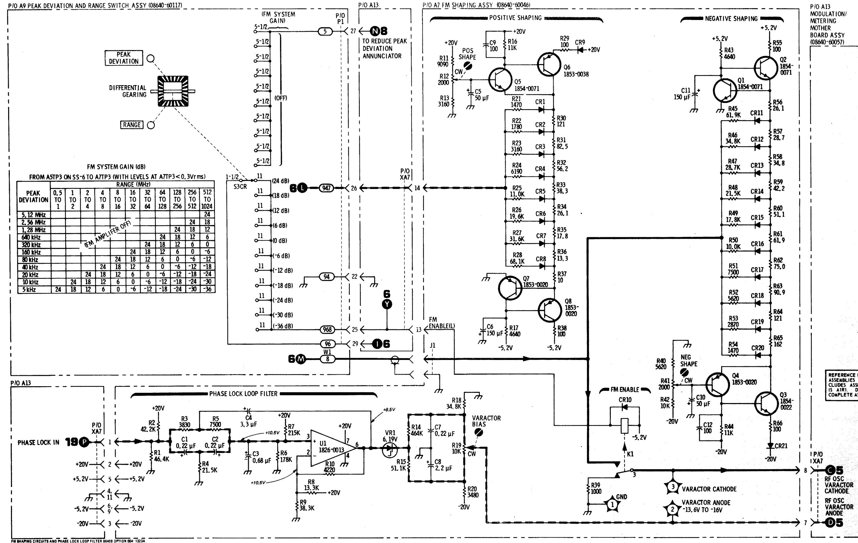
Figure 8-29. FM Shaping Circuits and Phase Lock Loop Filter Schematic Diagram
